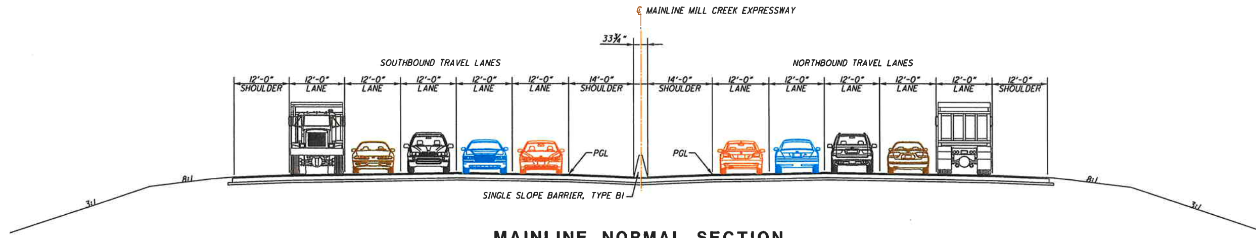
MAINLINE NORMAL SECTION MILL CREEK EXPRESSWAY 5 - LANE ALTERNATIVE
